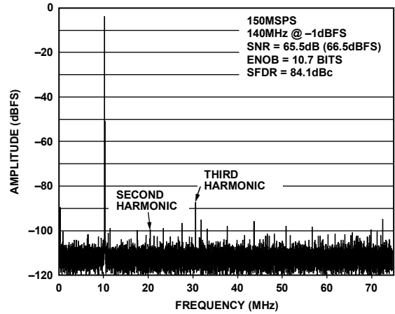
Figure 19. AD9627-11-150 Single-Tone FFT with f_{IN} = 140 MHz
