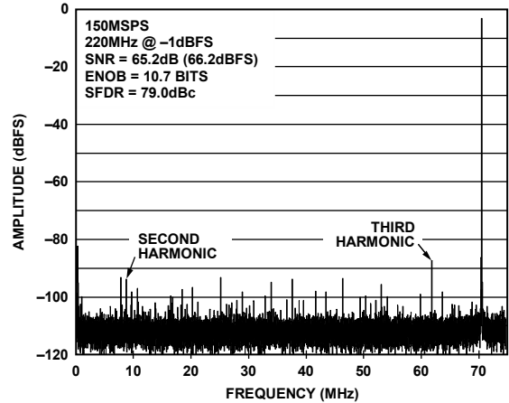
Figure 20. AD9627-11-150 Single-Tone FFT with f_{IN} = 220 MHz
