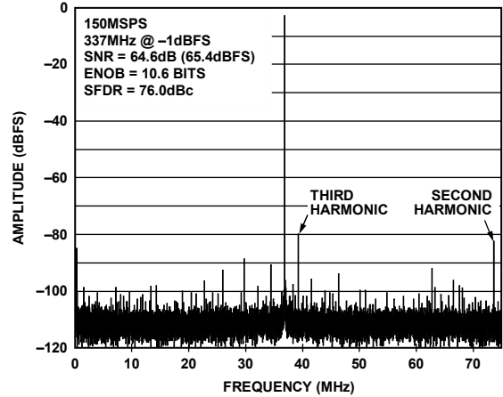
Figure 21. AD9627-11-150 Single-Tone FFT with f_{IN} = 337 MHz
