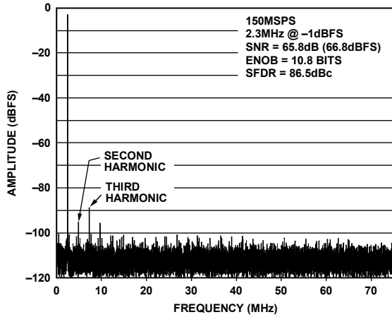
Figure 16. AD9627-11-150 Single-Tone FFT with f_{IN} = 2.3 MHz
